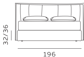
196 materasso largh. cm. 160 mattress width cm. 160
