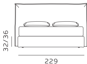
229 materasso largh. cm. 193 mattress width cm. 193
