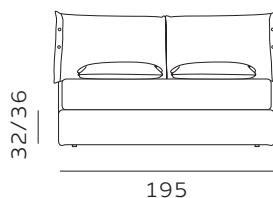
32/36 195 materasso largh. cm. 160 mattress width cm. 160
