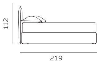
219 materasso lungh. cm. 203 mattress length cm. 203
